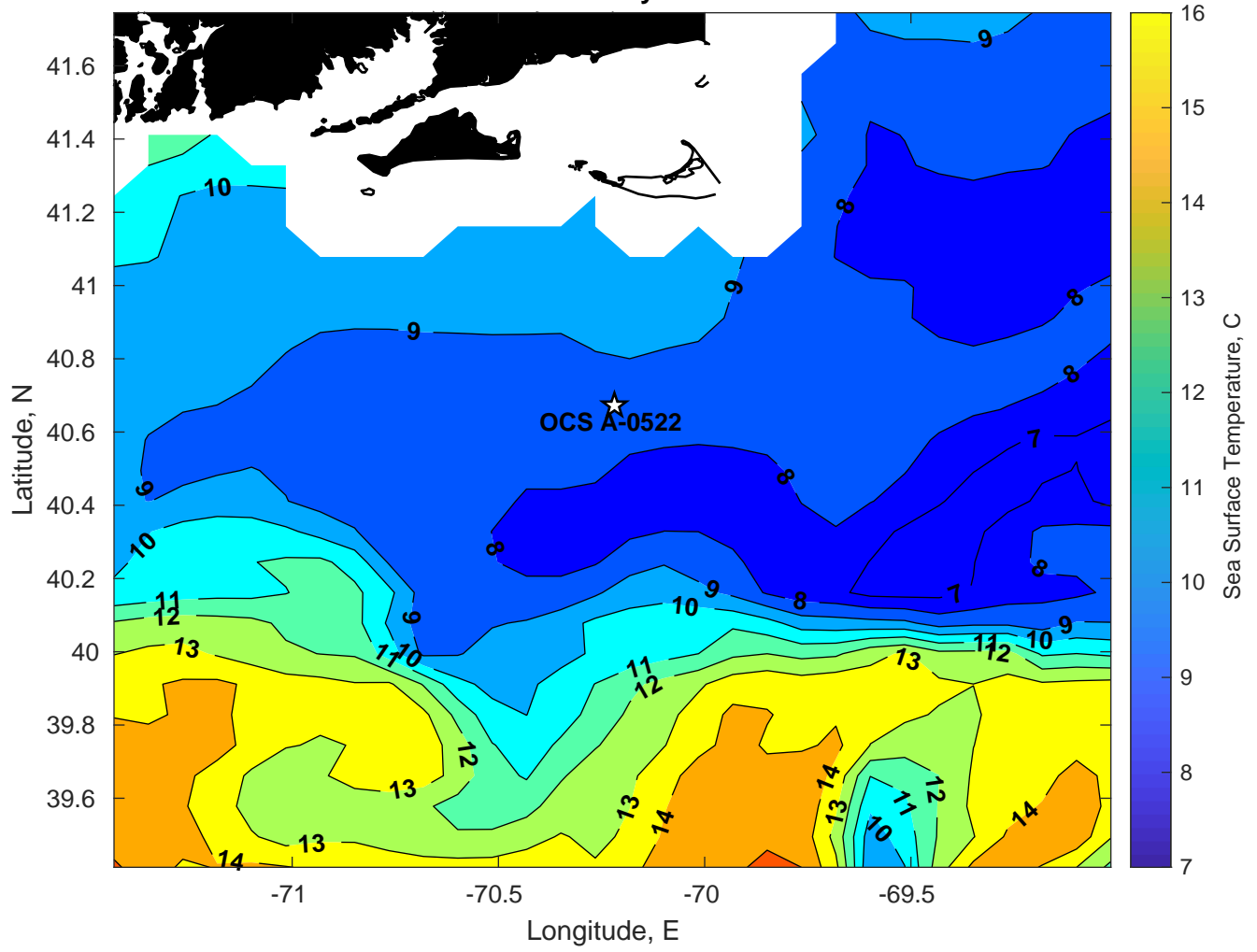
SST for OCS A-0522 at 18-May-2024 00:00:00
